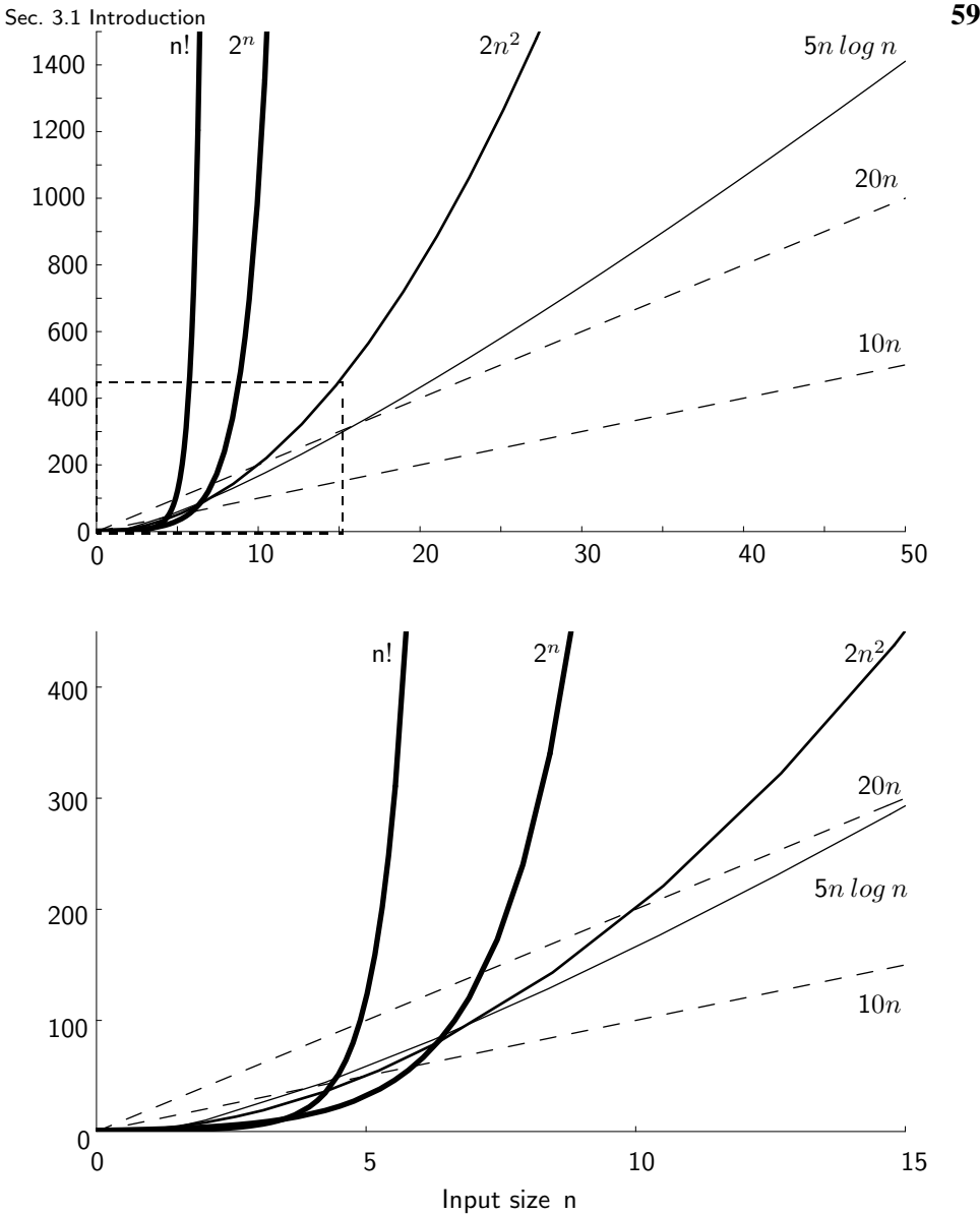
Figure 3.1 Two views of a graph illustrating the growth rates for six equations. The bottom view shows in detail the lower-left portion of the top view. The horizontal axis represents input size. The vertical axis can represent time, space, or any other measure of cost.
